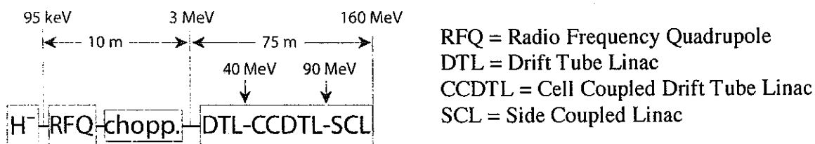
Figure 1: Basic structure of LINAC4
